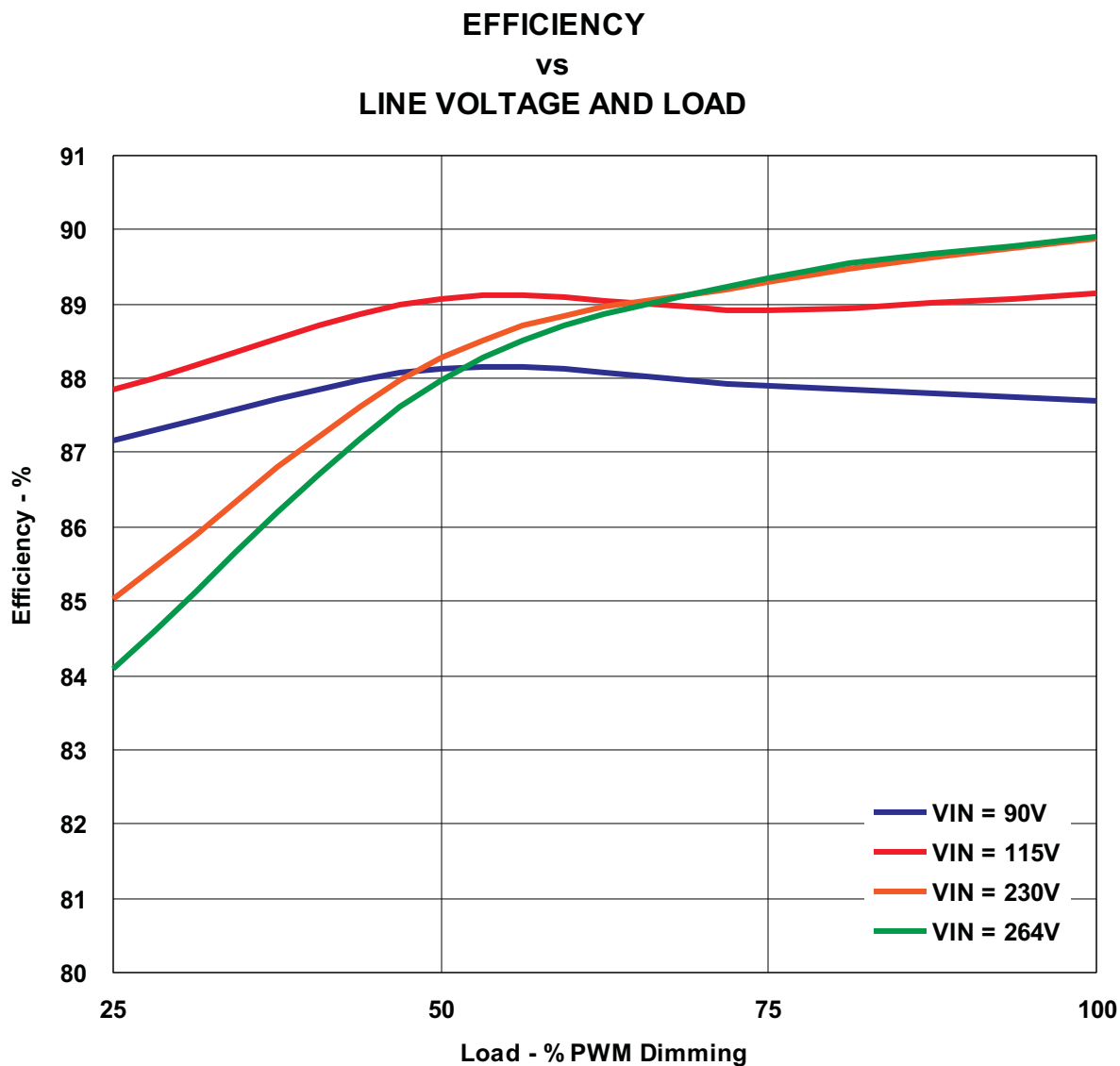
Figure 7. 4 x 15 Cree XRE LED's at 500 mA
