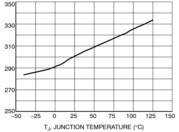
Figure 27. Inhibit Bias Current vs. Junction Temperature
