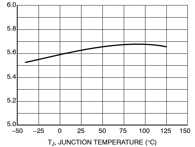
Figure 29. Startup Current vs. Junction Temperature
