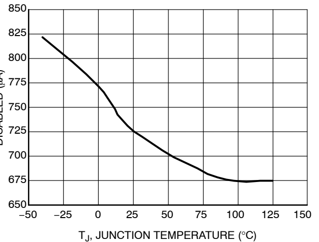
Figure 31. Supply Current Device Disabled (Overload) vs. Junction Temperature
