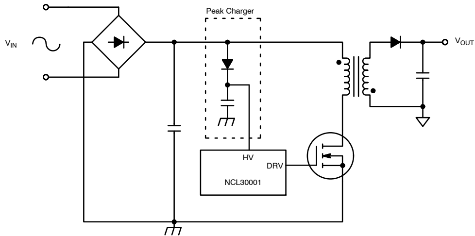
Figure 52. Peak charger
