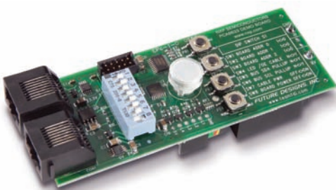
The PCA9633 demo board drives and mixes four LED colors (RGBA) to easily demonstrate networked I 2 C for signage and architectural lighting applications; order number OM6276
